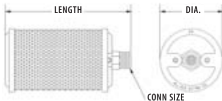
Single Chamber-Male
